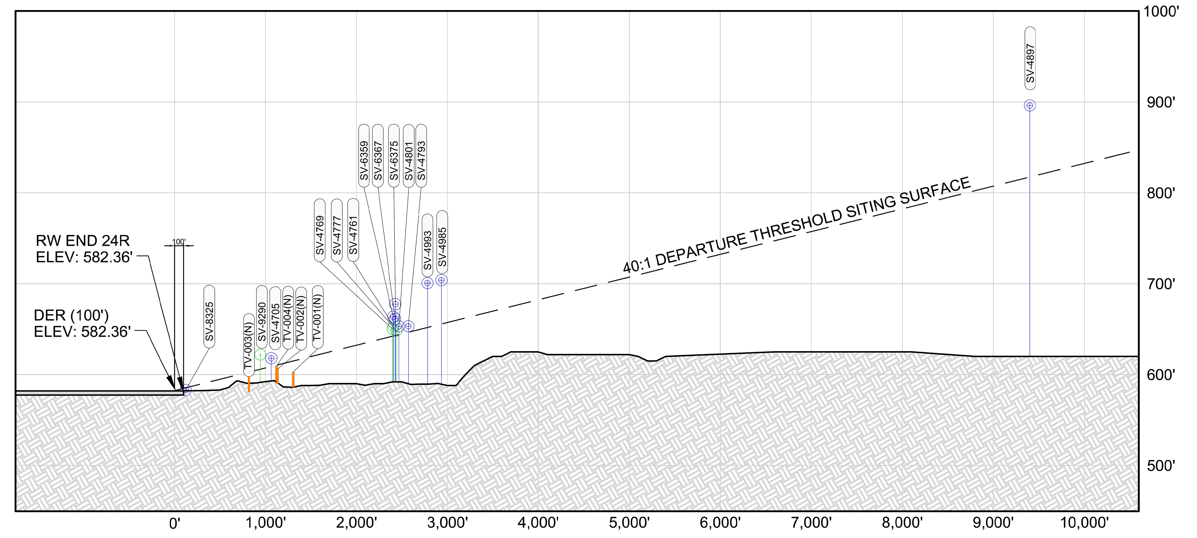
RUNWAY 6L DEPARTURE SURFACE - PROFILE VIEW SCALE: AS SHOWN
