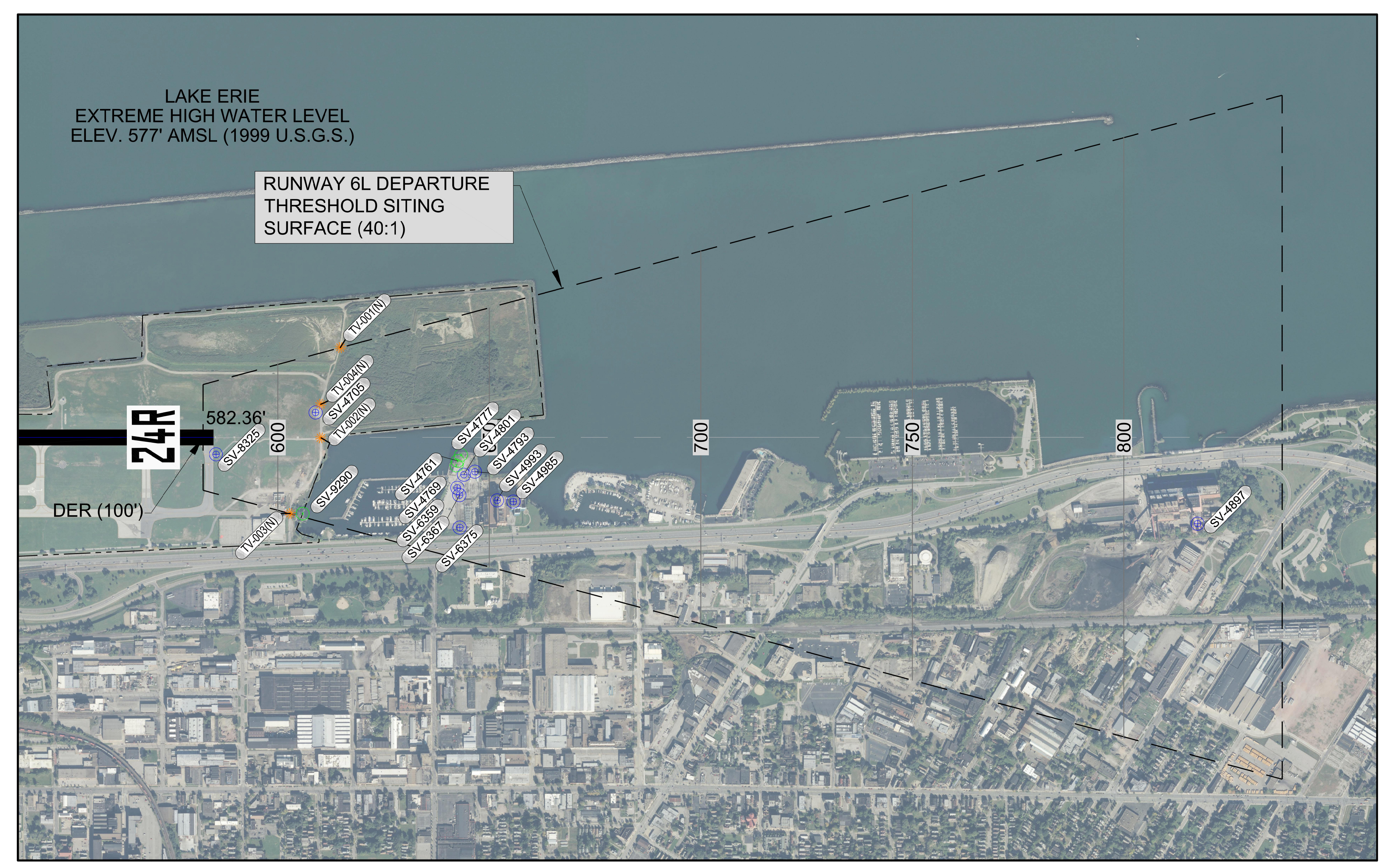
RUNWAY 6L DEPARTURE SURFACE - PLAN VIEW SCALE: 1"=600'
